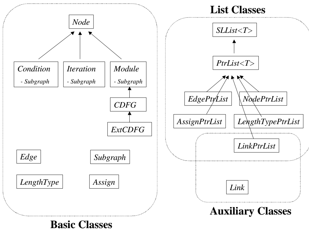
Figure 4. Class hierarchy of CDFG parser.
